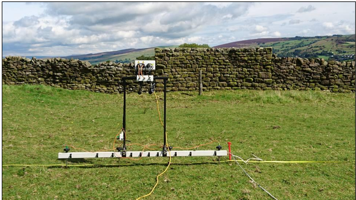
Figure 5-Resistivity probes in the foreground with the Malkin Gable in the background.
